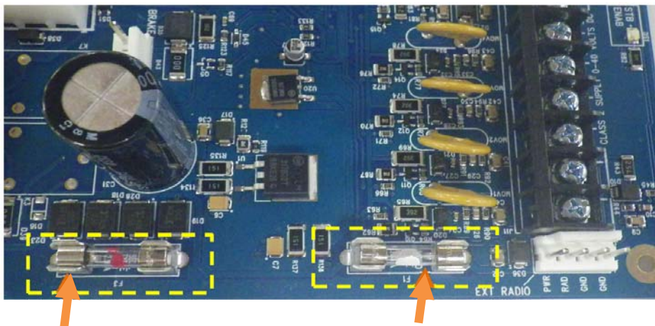
Position F3: Red Fuse
