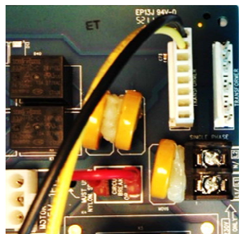
1ph Circuit Board with Harness
