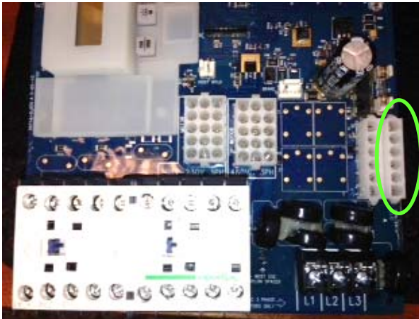
3ph Circuit Board
