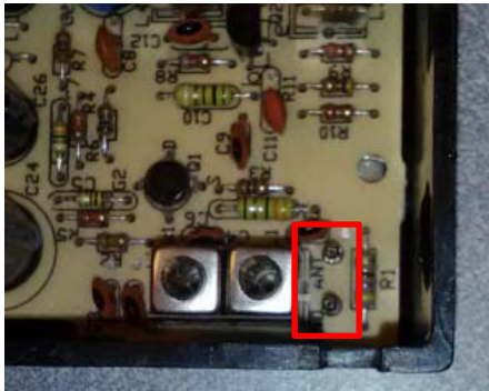
Pin Posts in Receiver that Connectors on Coax Cable Plug Into
